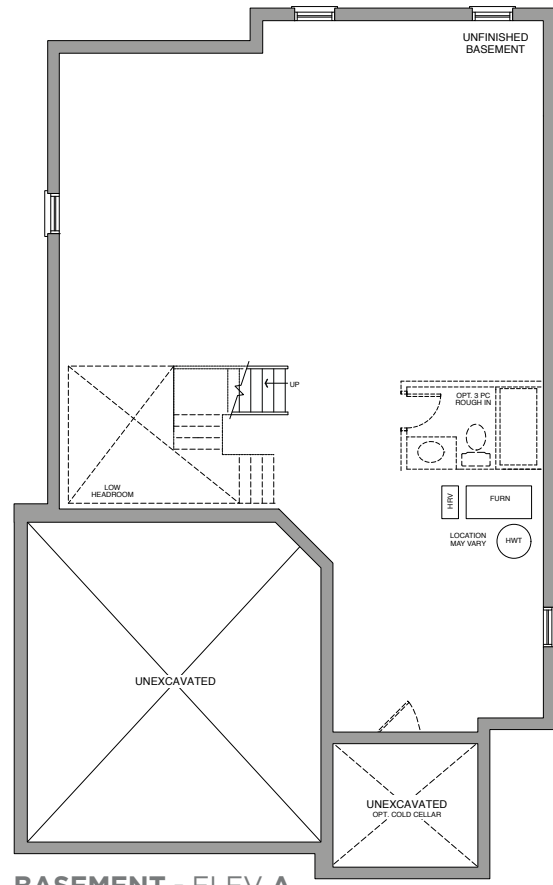
BASEMENT - ELEV A
