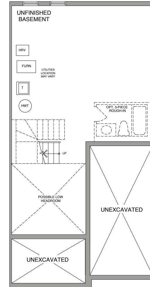
BASEMENT - ELEV A & B
