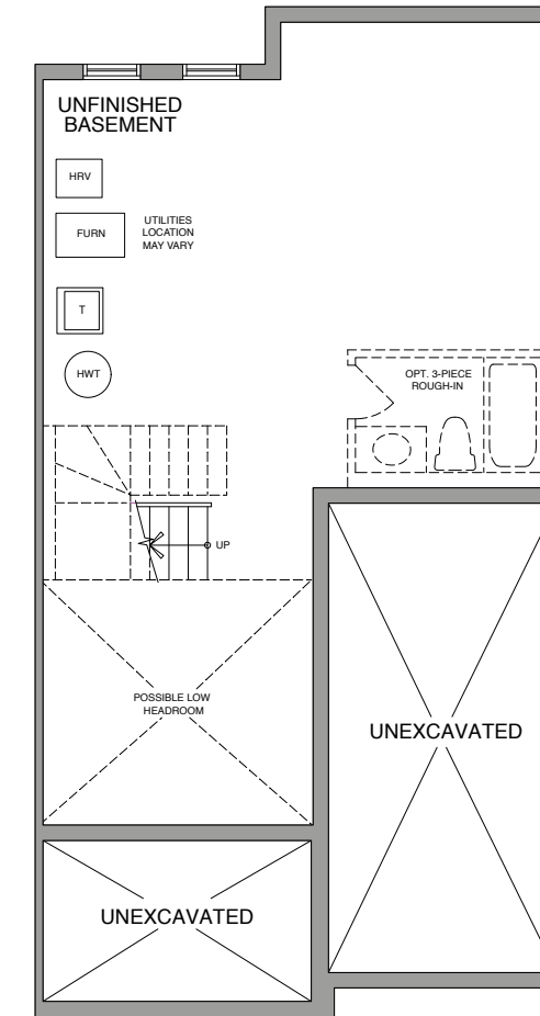
BASEMENT - ELEV A & B
