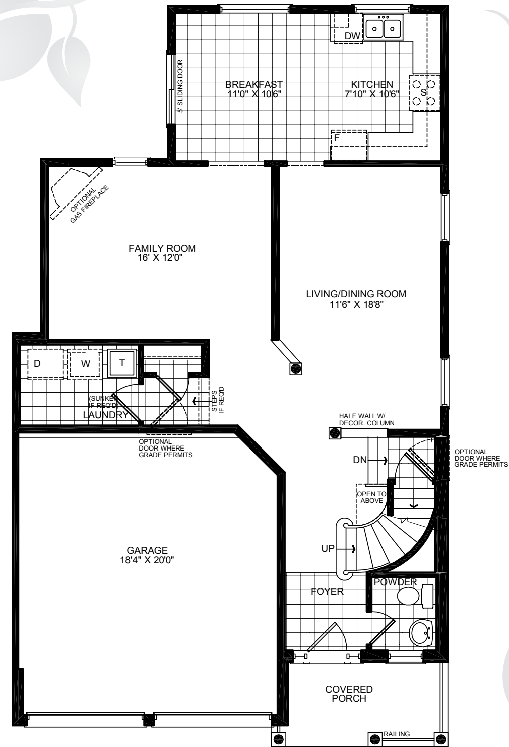
Ground floor
