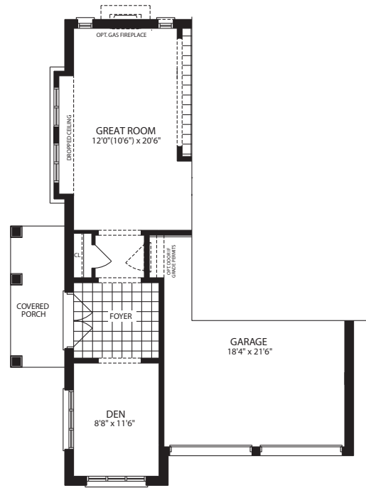
PART. GROUND FLOOR ELEVATION 'B'
