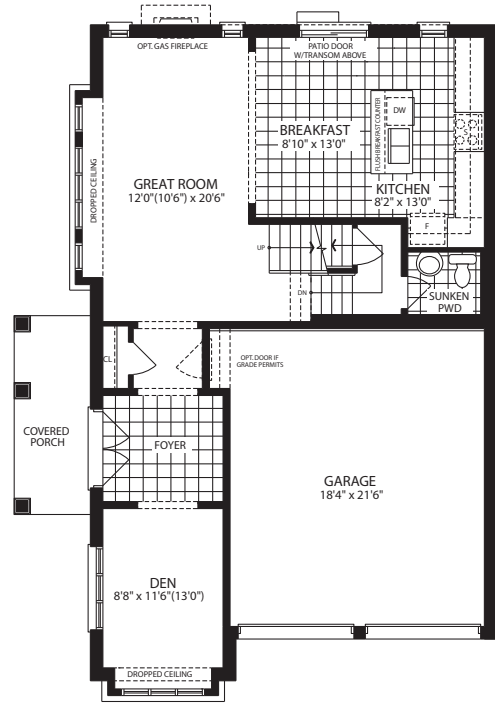
GROUND FLOOR ELEVATION 'A'
