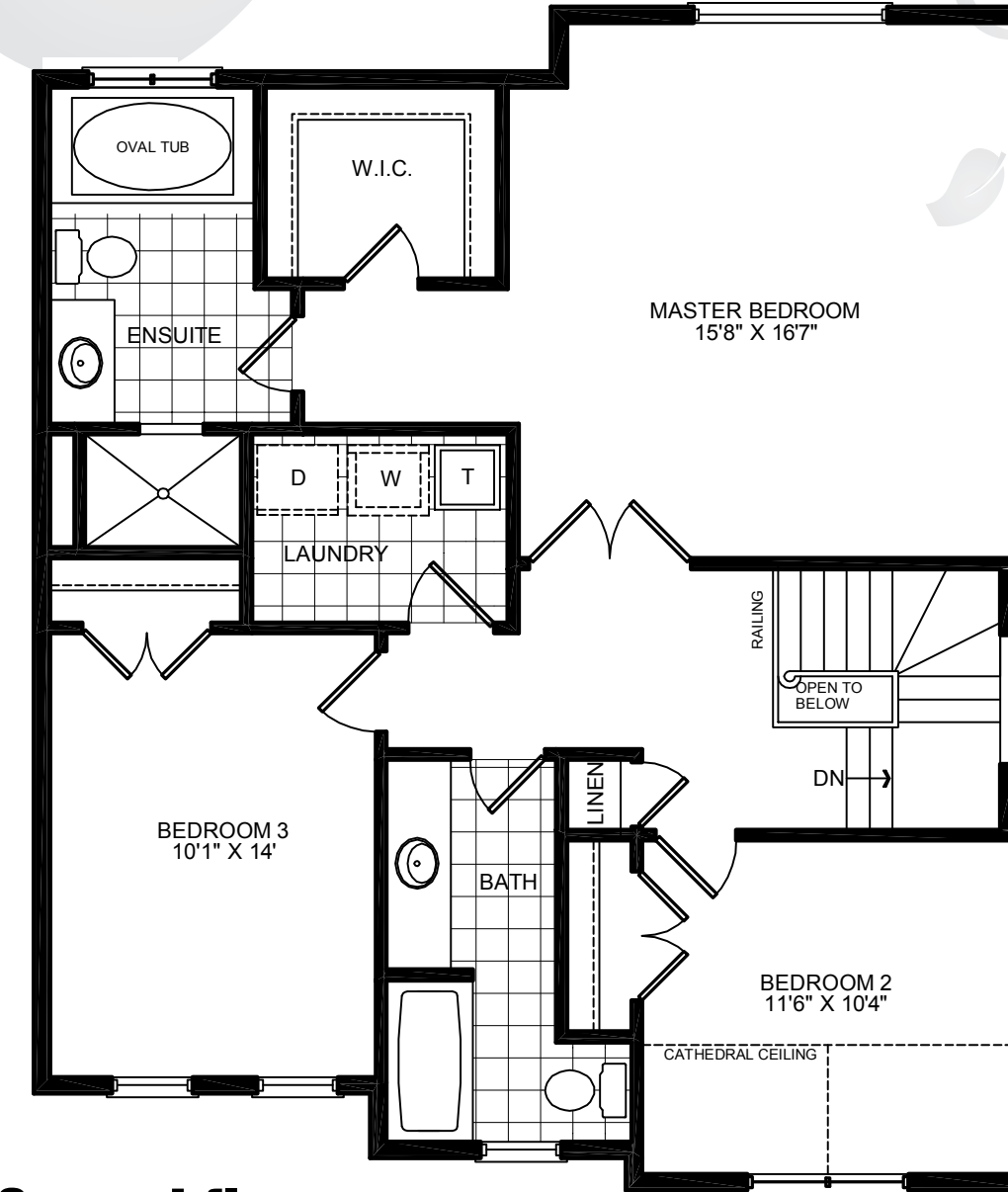
Second floor
